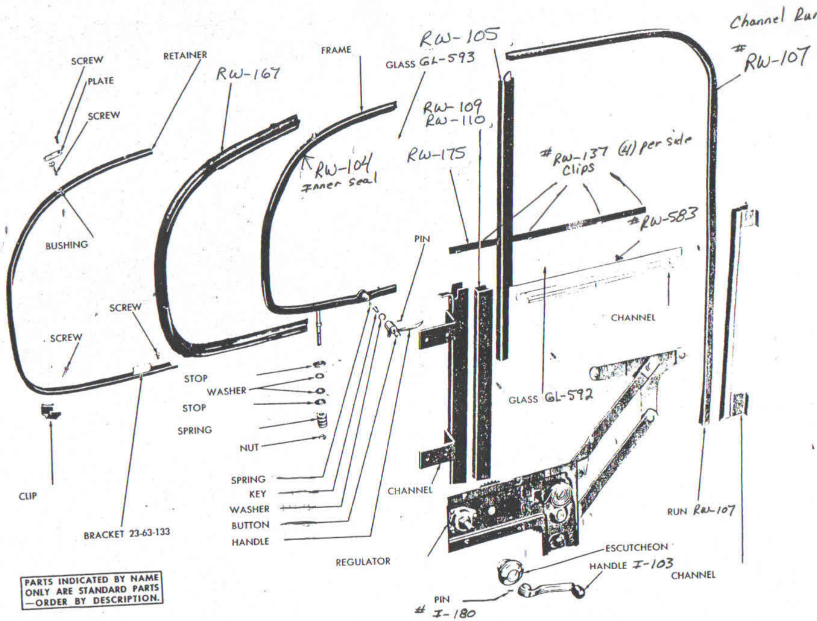
DOOR GLASS REGULATOR AND RUNS (EXPLODED VIEW)
